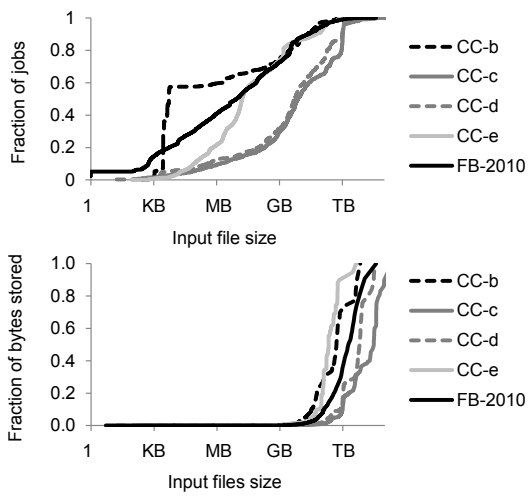
Figure 3: Access patterns vs. input file size. Showing cumulative fraction of jobs with input files of a certain size (top) and cumulative fraction of all stored bytes from input files of a certain size (bottom).
