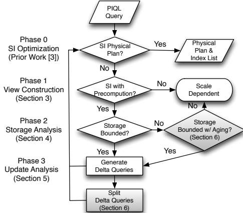
Figure 1: The phases of the scale-independent optimizer and view selection system.
