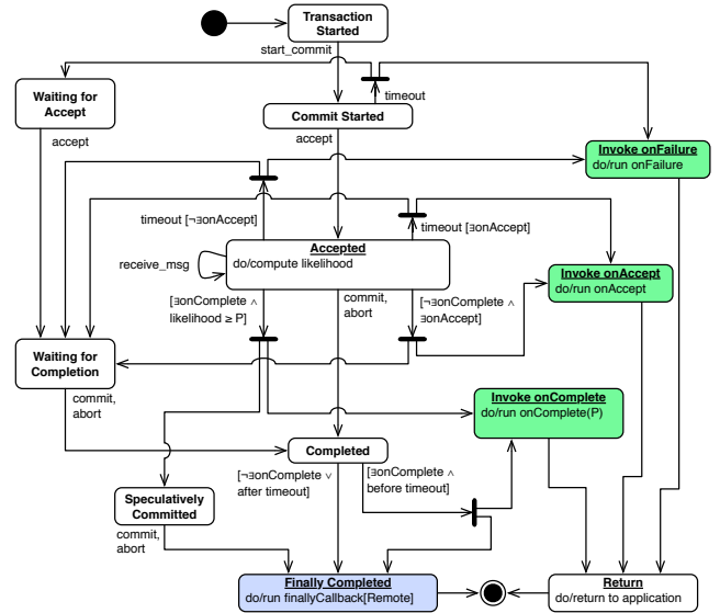
Figure 3: PLANET transaction state diagram
