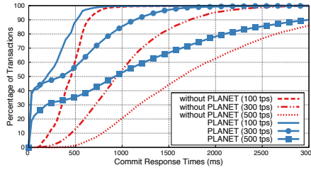
Figure 9: Commit response time CDF (50,000 items, 100 hotspot)
