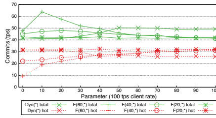
Figure 12: Admission control, vary policies (100 TPS, 25,000 items, 50 hotspot)
