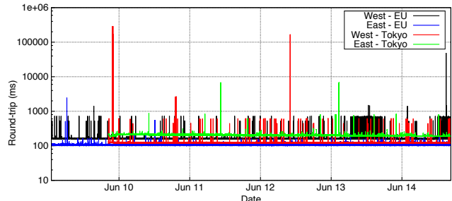
Figure 1: Round trip response times between various regions on Amazon's EC2 cluster.
