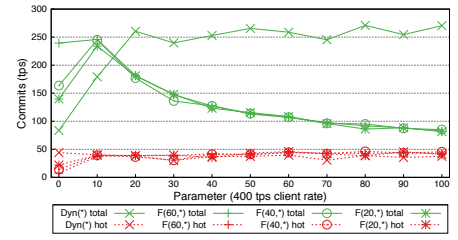
Figure 13: Admission control, vary policies (400 TPS, 25,000 items, 50 hotspot)
