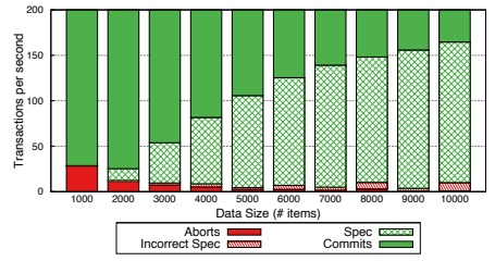
Figure 10: Transaction types, vary data size (200 TPS, uniform access)
