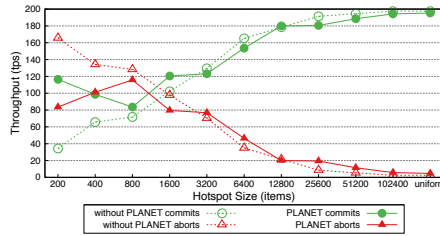
Figure 6: Commit & abort throughput, vary hotspot (200,000 items, 200 TPS)
