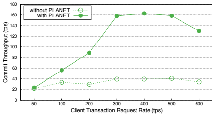
Figure 8: Commit throughput, vary client rate (50,000 items, 100 hotspot)
