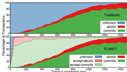
Figure 5: Transaction outcomes, vary timeout (20,000 items, 200 TPS)
