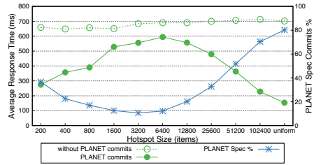
Figure 7: Average response time, vary hotspot (200,000 items, 200 TPS)
