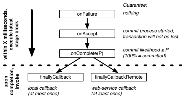
Figure 2: Client view of PLANET transactions
