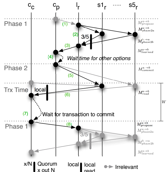
Figure 4: Time-sequence for rounds
