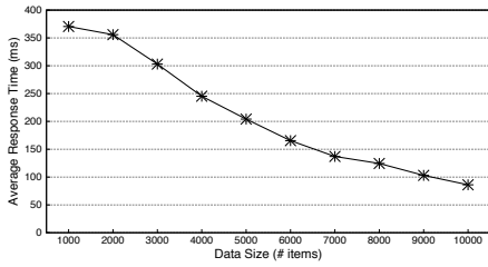
Figure 11: Average commit latency, vary data size (200 TPS, uniform access)
